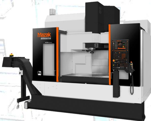
MAZAK vcn-530VCN-530c SG = 1 MACHINE X = 1,050 mm. Y = 530 mm. Z = 510 mm.
